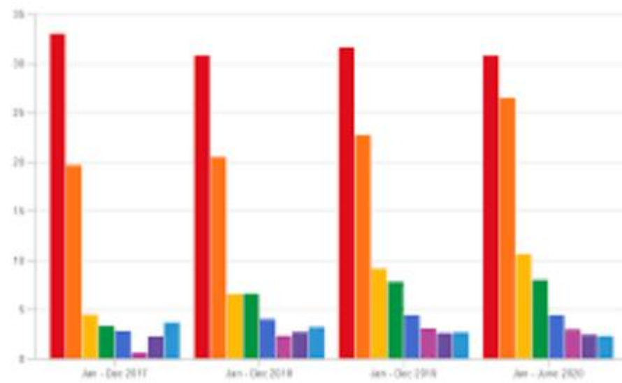
Fig 1. Monthly Rainfall
